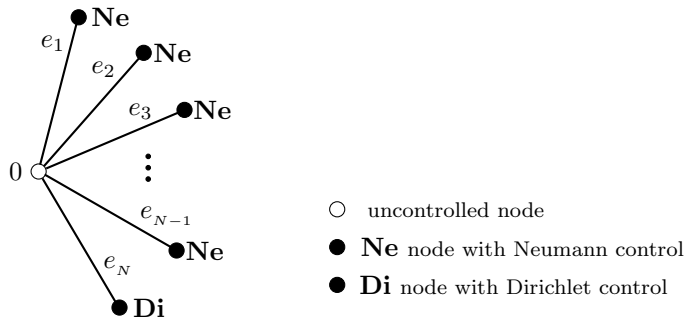
FIG. 3. Network with N edges for m = N - 1 .
