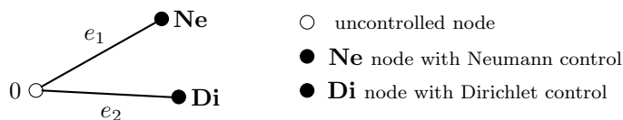
FIG. 1. Network with 2 edges and mixed controls.
