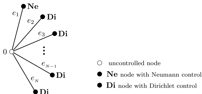
FIG. 2. Network with N edges for m = 1 .
