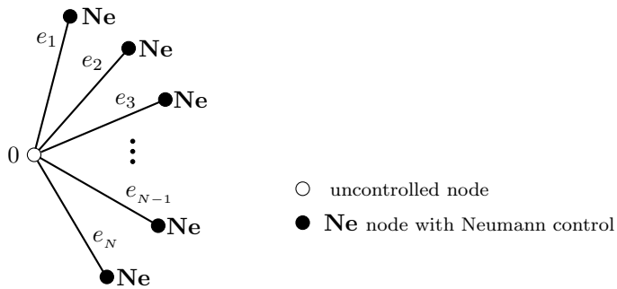
FIG. 5. Network with N edges with control on Neumann condition.
