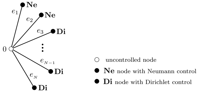
FIG. 4. Network with N edges for m = 2 .
